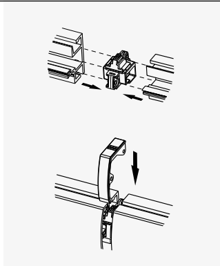
① Connection of profiles
