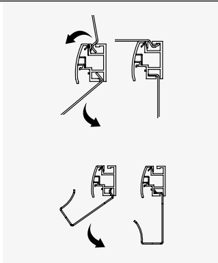
① Installation of accessories
